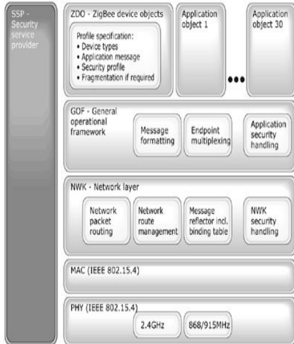
Fig.II.iii ZigBee protocol stack architecture
