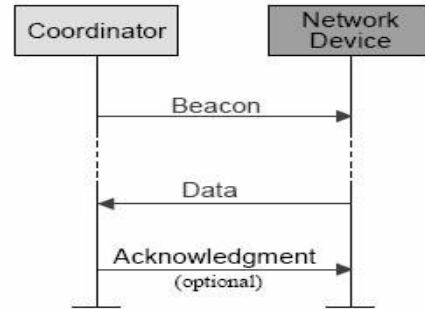
Figure III.i: Beacon Network Communication
