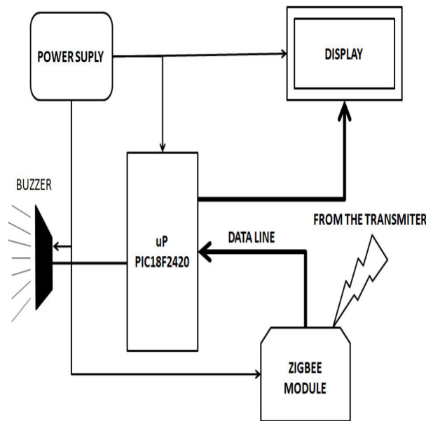
Figure II.ii: receiver module
