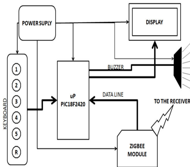
Figure II.i: transmitter module
