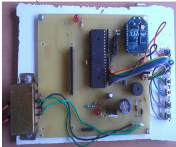
Figure IV.ii circuit of receiver module
